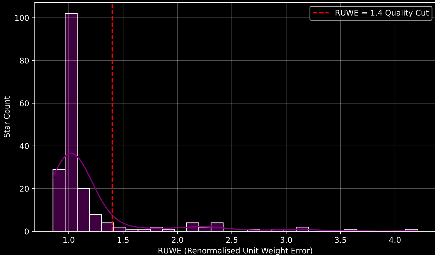
GAPOGEE DR17 Field [077+69_MGA] RUWE Distribution (n= 187)
