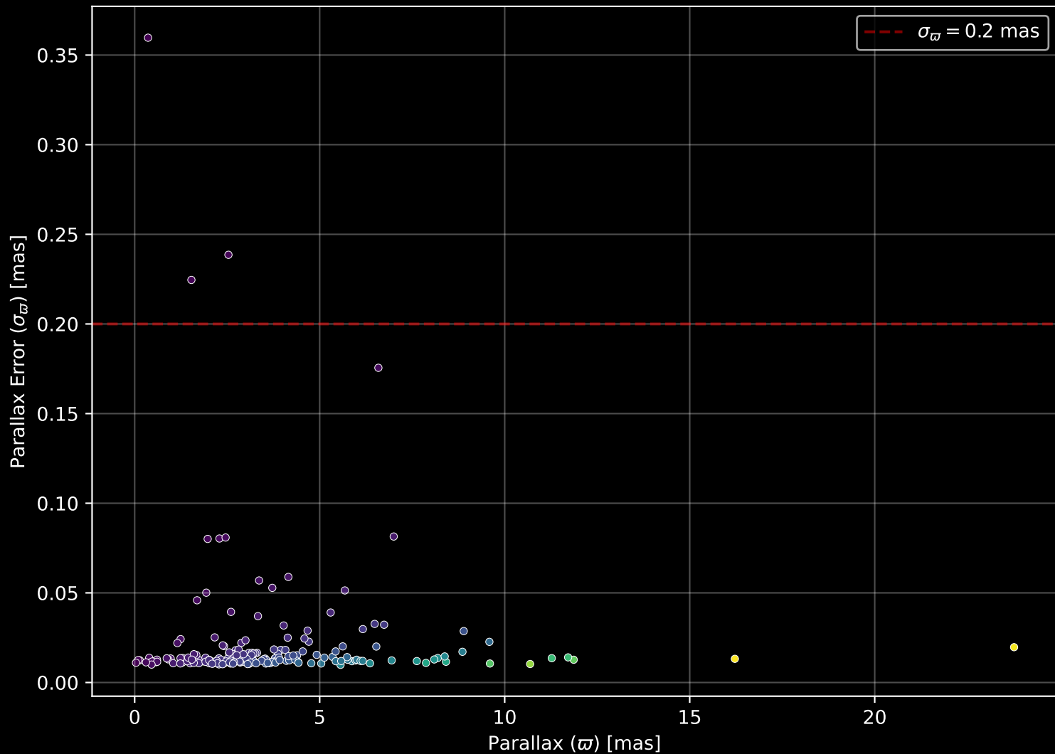
APOGEE DR17 Field: [077+69_MGA] Parallax Quality (n= 196)
