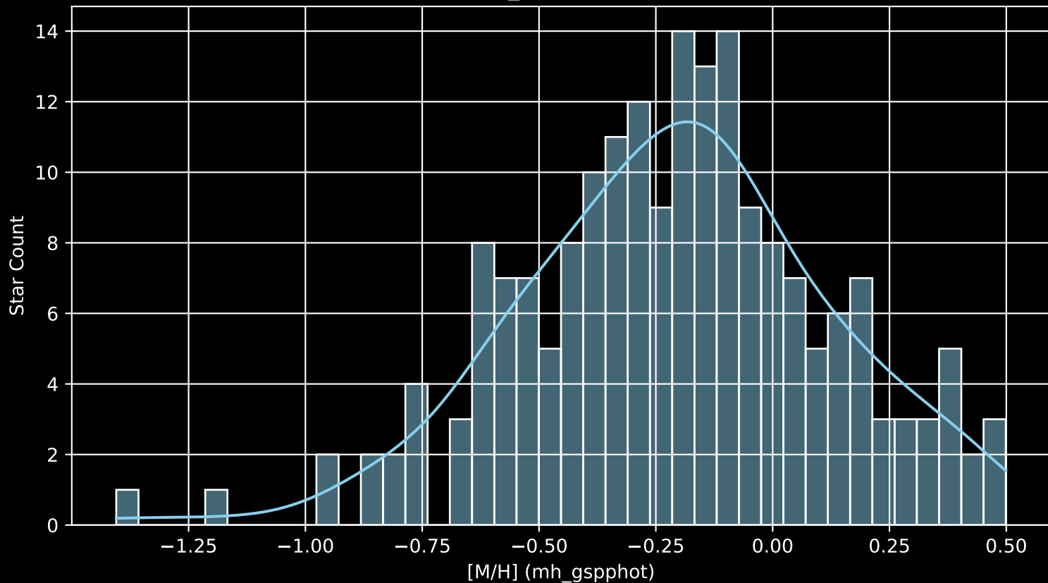
APOGEE DR17 Field: [077+69_MGA [M/H] (mh_gspphot) (n= 194)
