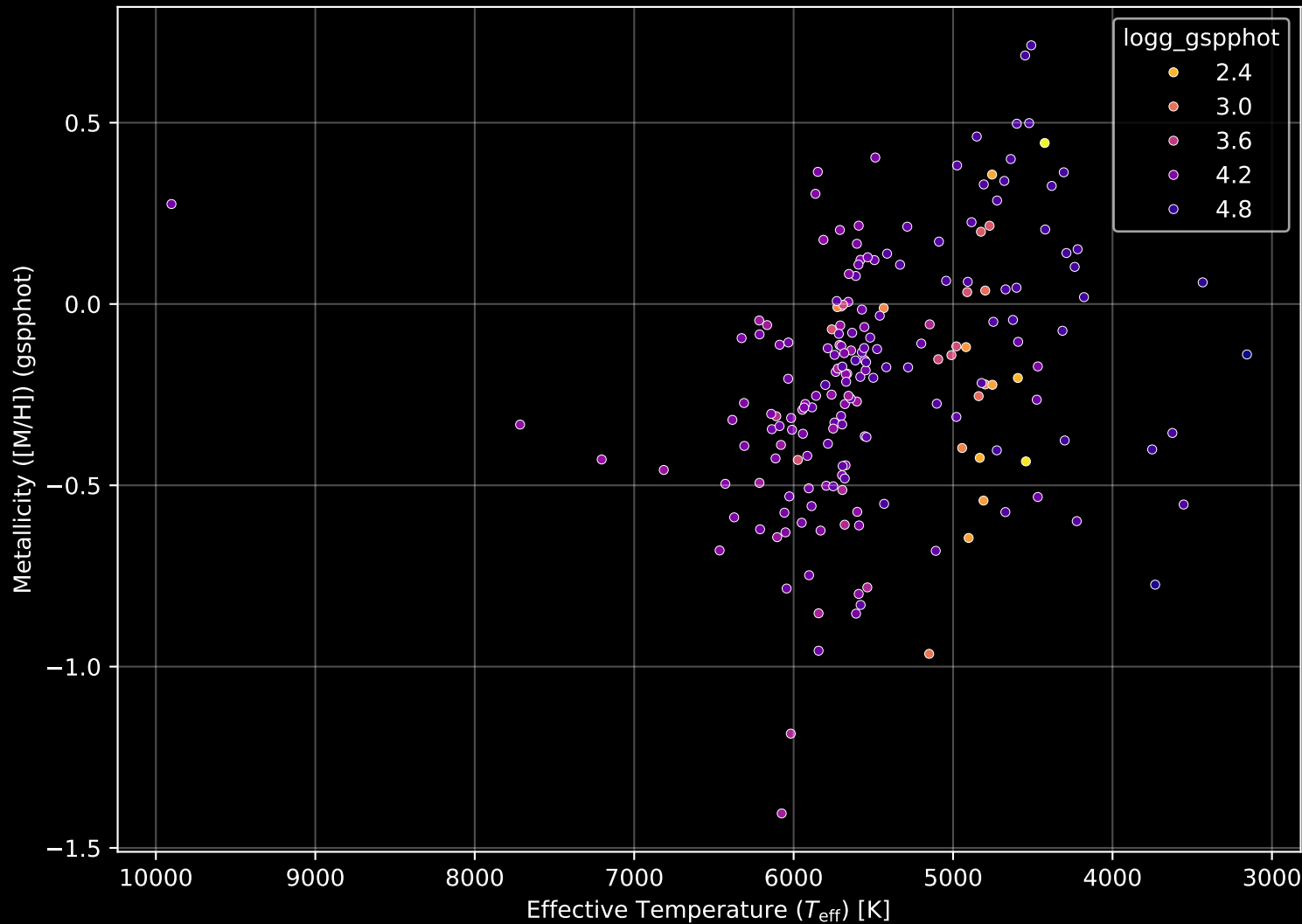
APOGEE DR17 Field: [077+69_MGA] Stellar Population Parameters (n= 196)
