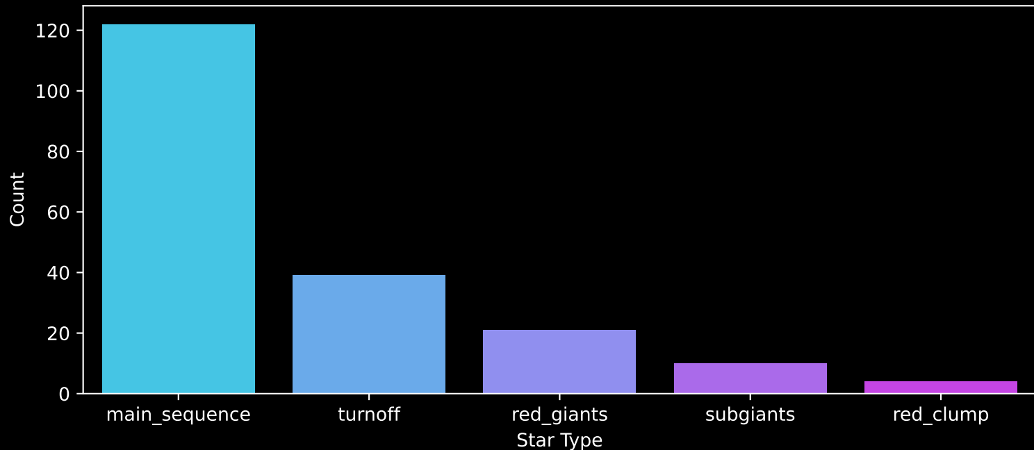
APOGEE DR17 Field: [077+69_MGA] Count plot of Star Type
