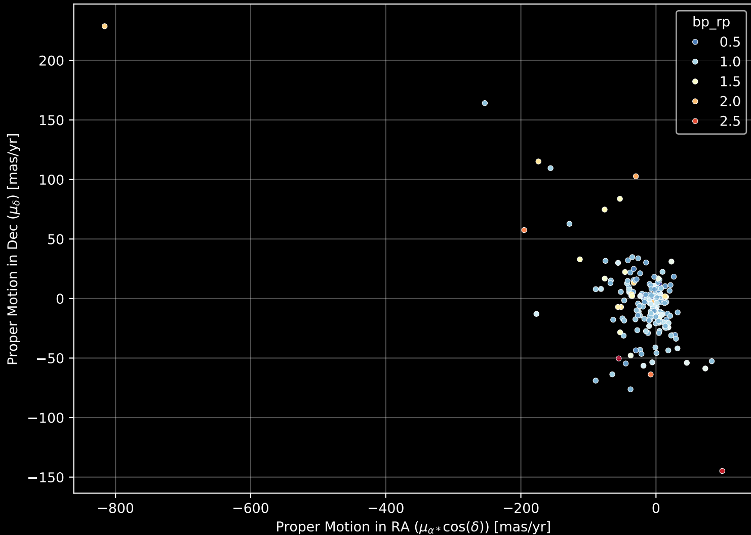
APOGEE DR17 Field: [077+69_MGA] Proper Motion Diagram (n = 196)
